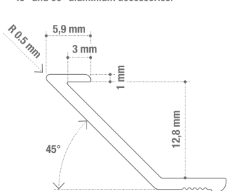
Accessori alluminio 45° e 90°. 45° and 90° aluminium accessories.
